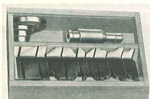
No. 1184 Set of Sash and Cabinet Cutters, Collars, Spindle and Wrench, in wood box.
